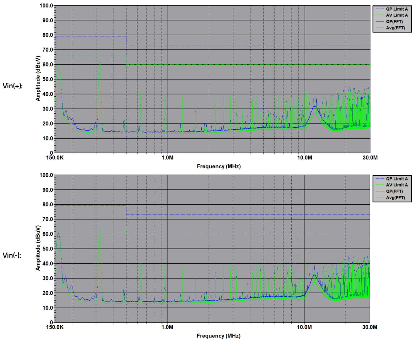
Figure 22. EMC Consideration
