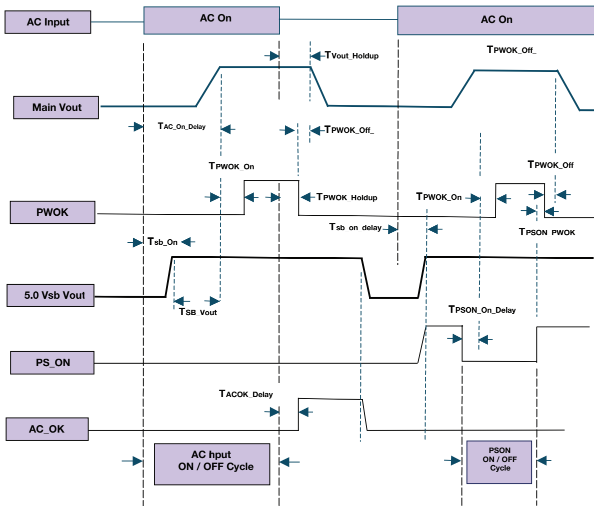
Timing Diagram
