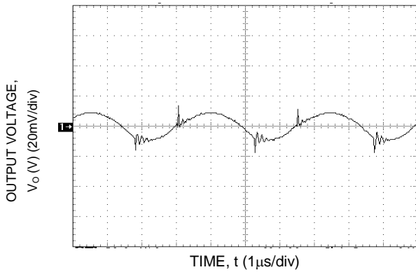
Figure 14. Typical Output Ripple and Noise.
