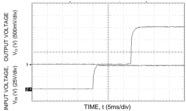
Figure 35. Typical Start-Up with application of Vin.
