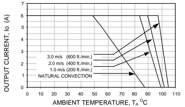
Figure 46. Derating Output Current versus Local Ambient Temperature and Airflow.
