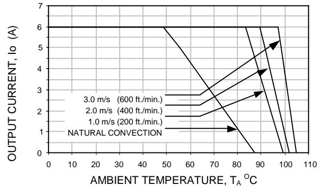
Figure 40. Derating Output Current versus Local Ambient Temperature and Airflow
