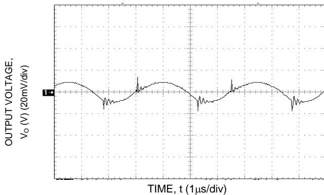
Figure 14. Typical Output Ripple and Noise.
