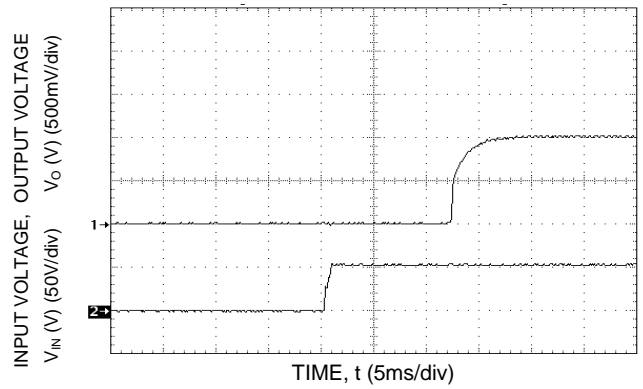
Figure 47. Typical Start-Up with application of Vin.
