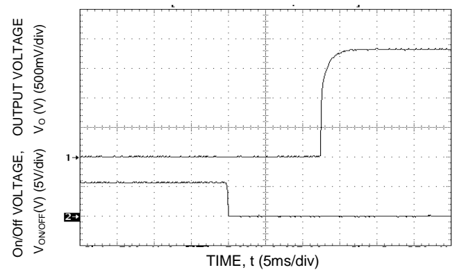
Figure 30. Typical Start-Up Using Remote On/Off, negative logic version shown.
