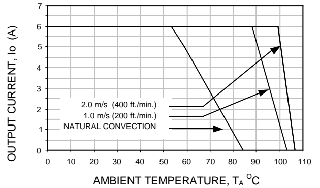
Figure 28. Derating Output Current versus Local Ambient Temperature and Airflow
