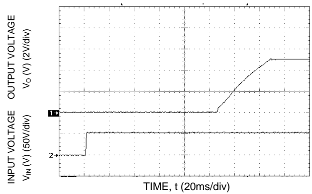
Figure 5. Typical Start-Up with application of Vin.
