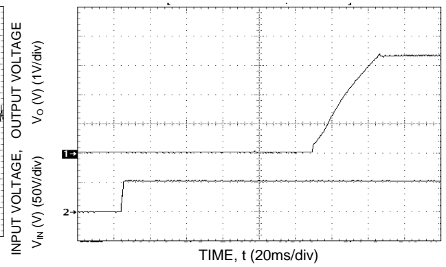
Figure 11. Typical Start-Up with application of Vin.
