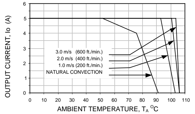
Figure 10. Derating Output Current versus Local Ambient Temperature and Airflow
