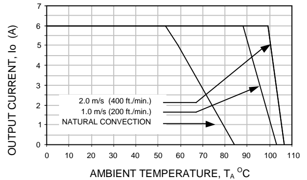
Figure 34. Derating Output Current versus Local Ambient Temperature and Airflow
