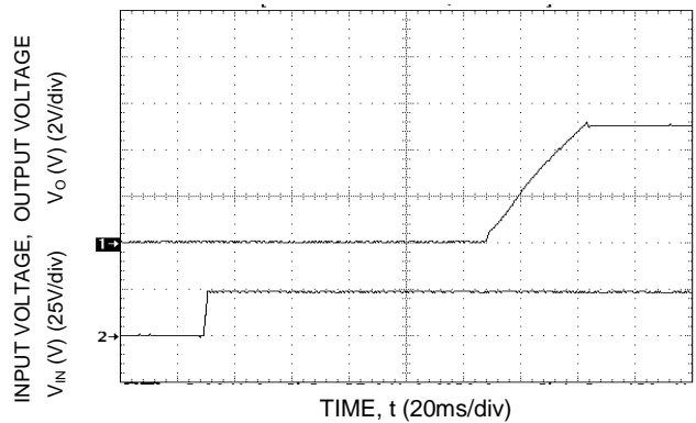
Figure 53. Typical Start-Up with application of Vin.
