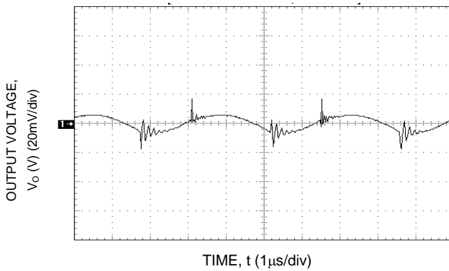
Figure 8. Typical Output Ripple and Noise.
